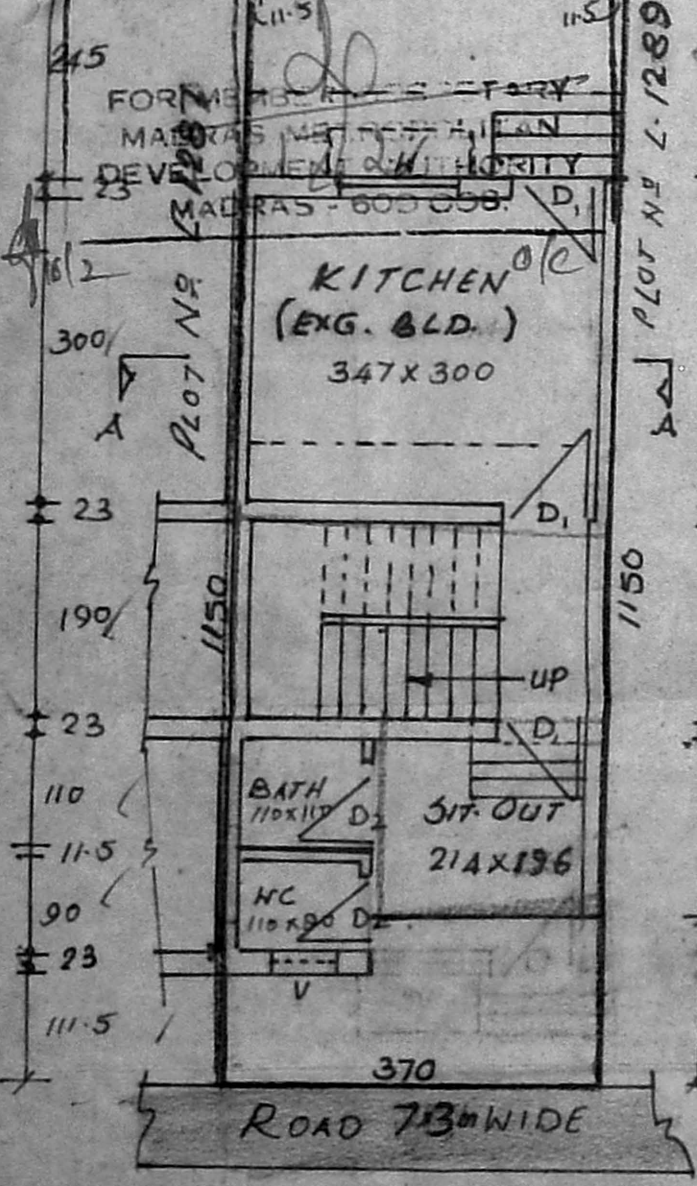
GROUND FLOOR PLAN & SITE PLAN
